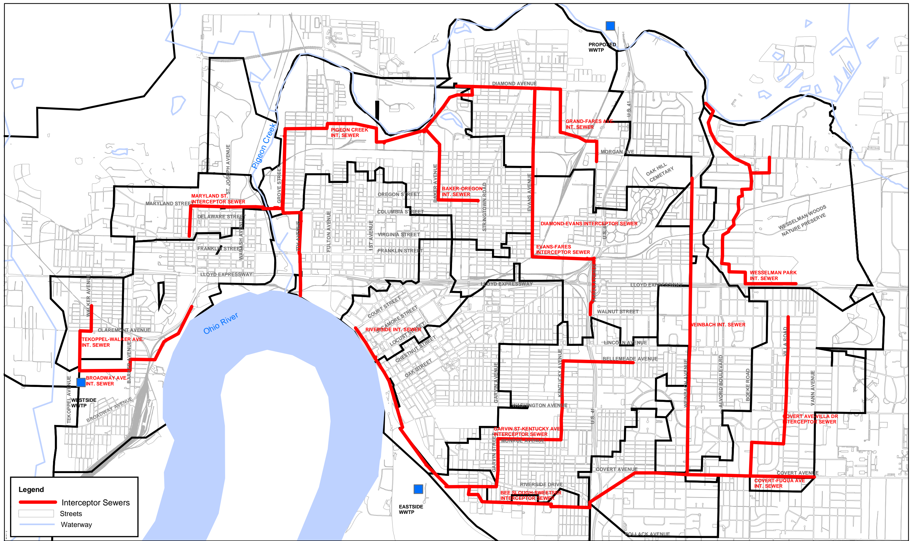
FIGURE 1.1 COMBINED SEWER AREA EVANSVILLE, INDIANA
